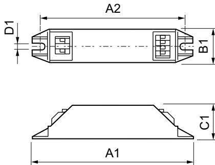
HF-M BLUE 124 LH TL/TL5/PL-L 230-240V
