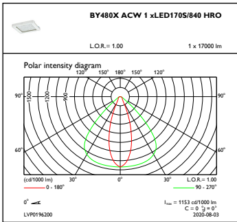
OFPC1_BY480XACW1xLED170S840HRO
