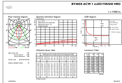
IFGU1_BY480XACW1xLED170S840HRO
