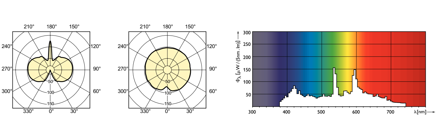
LDLD_CDM-T_0005-Light distribution diagram LDPO_CDM-T_35W_842-Spectral power distribution Colour
