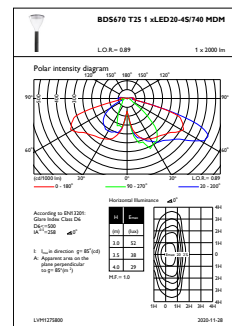
OFPL1_BDS670T251xLED20-4S740MDM
