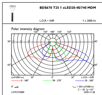
OFPC1_BDS670T251xLED20-4S740MDM
